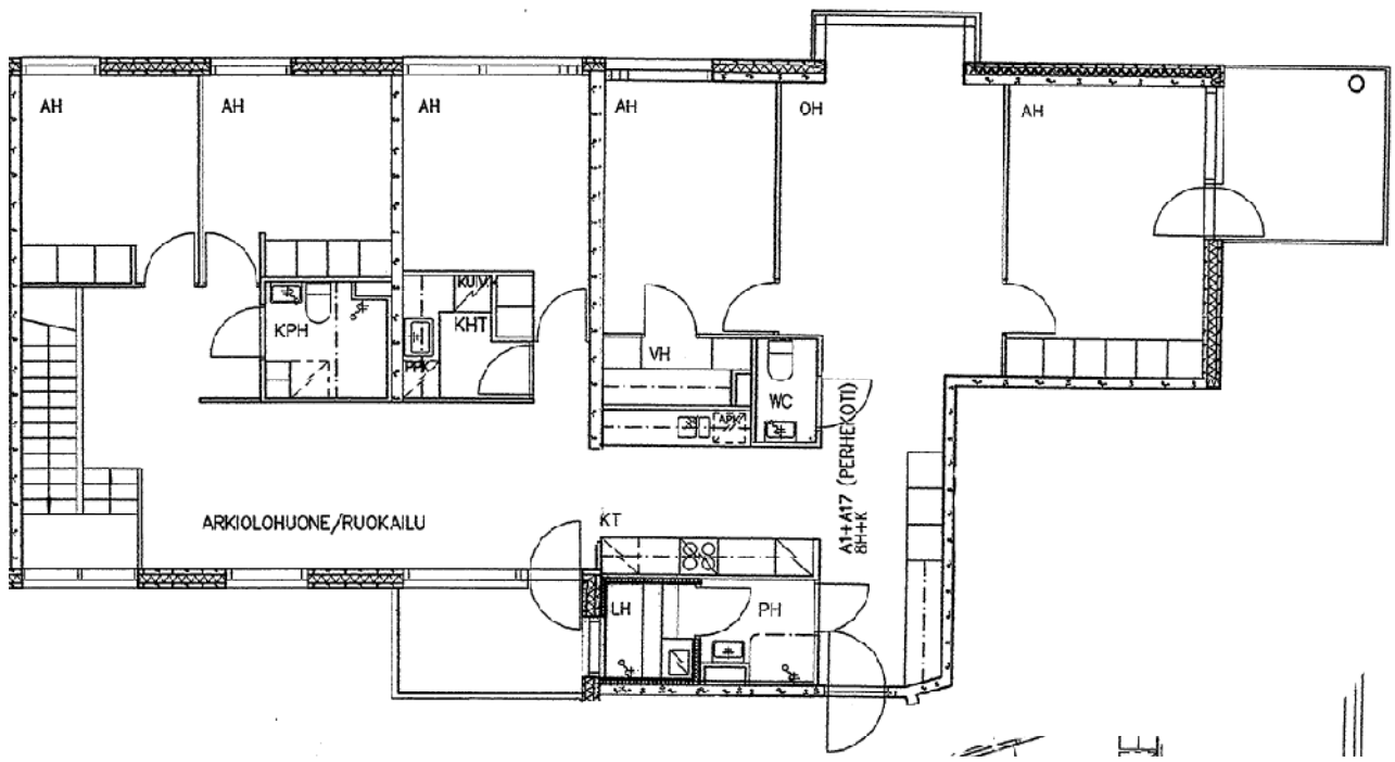
2. krs
