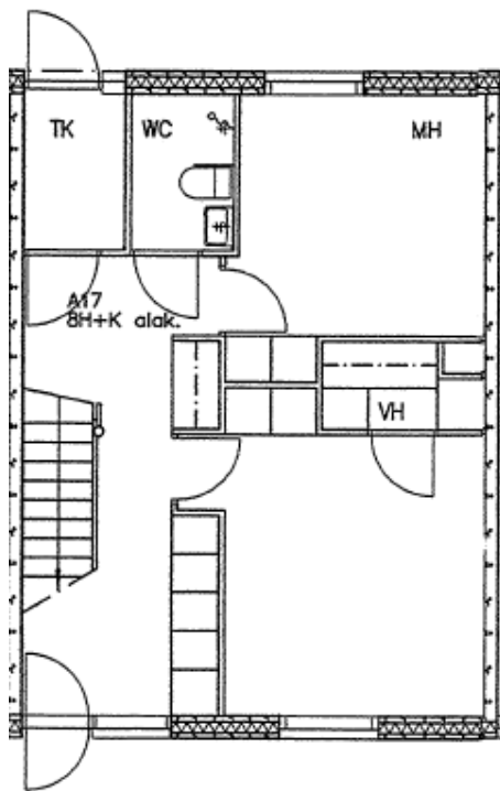
1. krs
